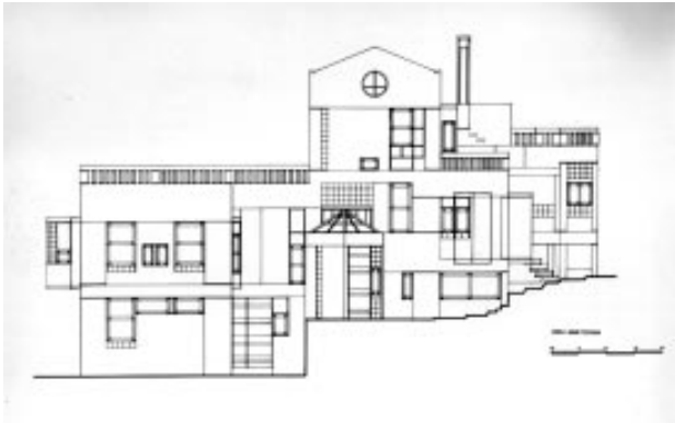
Tzitzikalakis Residence: East elevation
