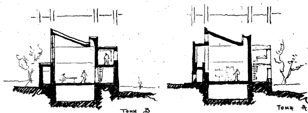
Mavrakakis Art Studio: Sections
