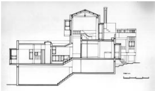
Tzitzikalakis Residence: Section
