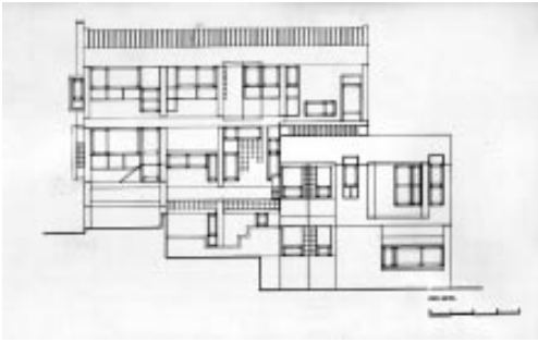
Tzitzikalakis Residence: South elevation
